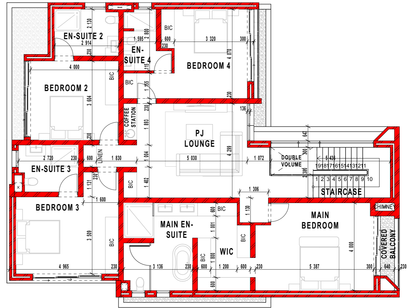
FIRST FLOOR Scale 1:100
