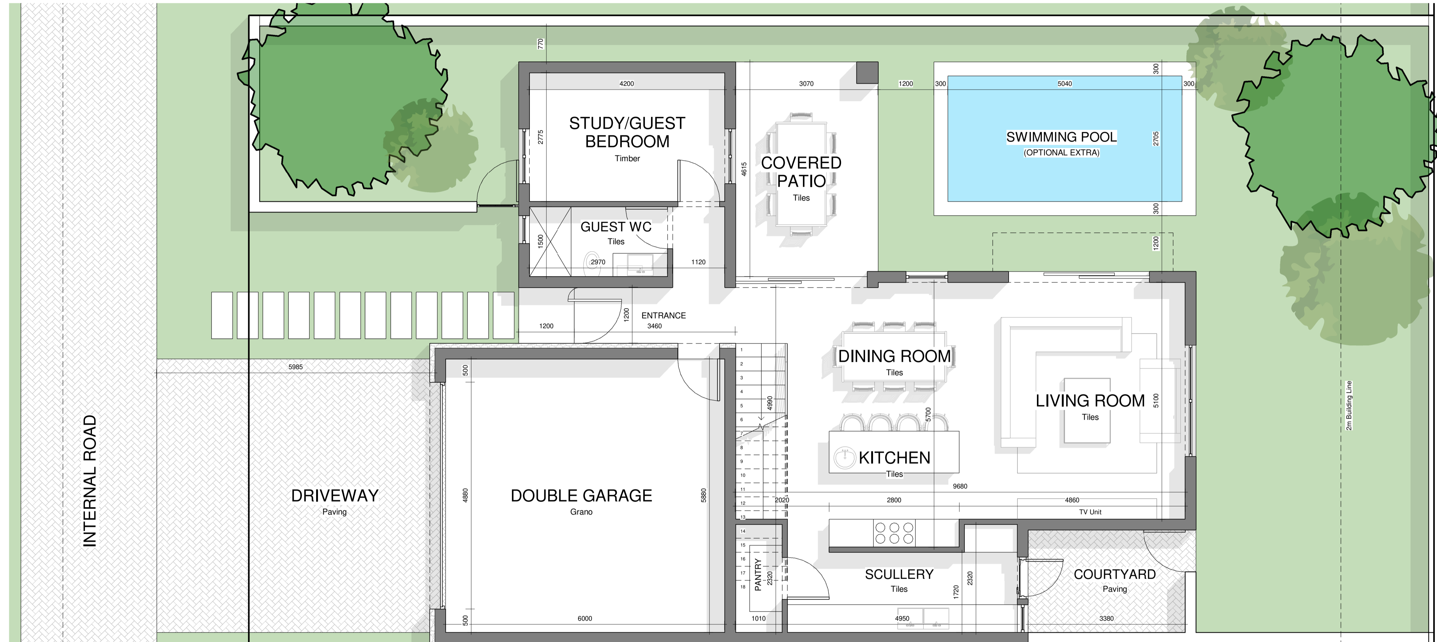
GROUND FLOOR_PTN 3 1 : 50
