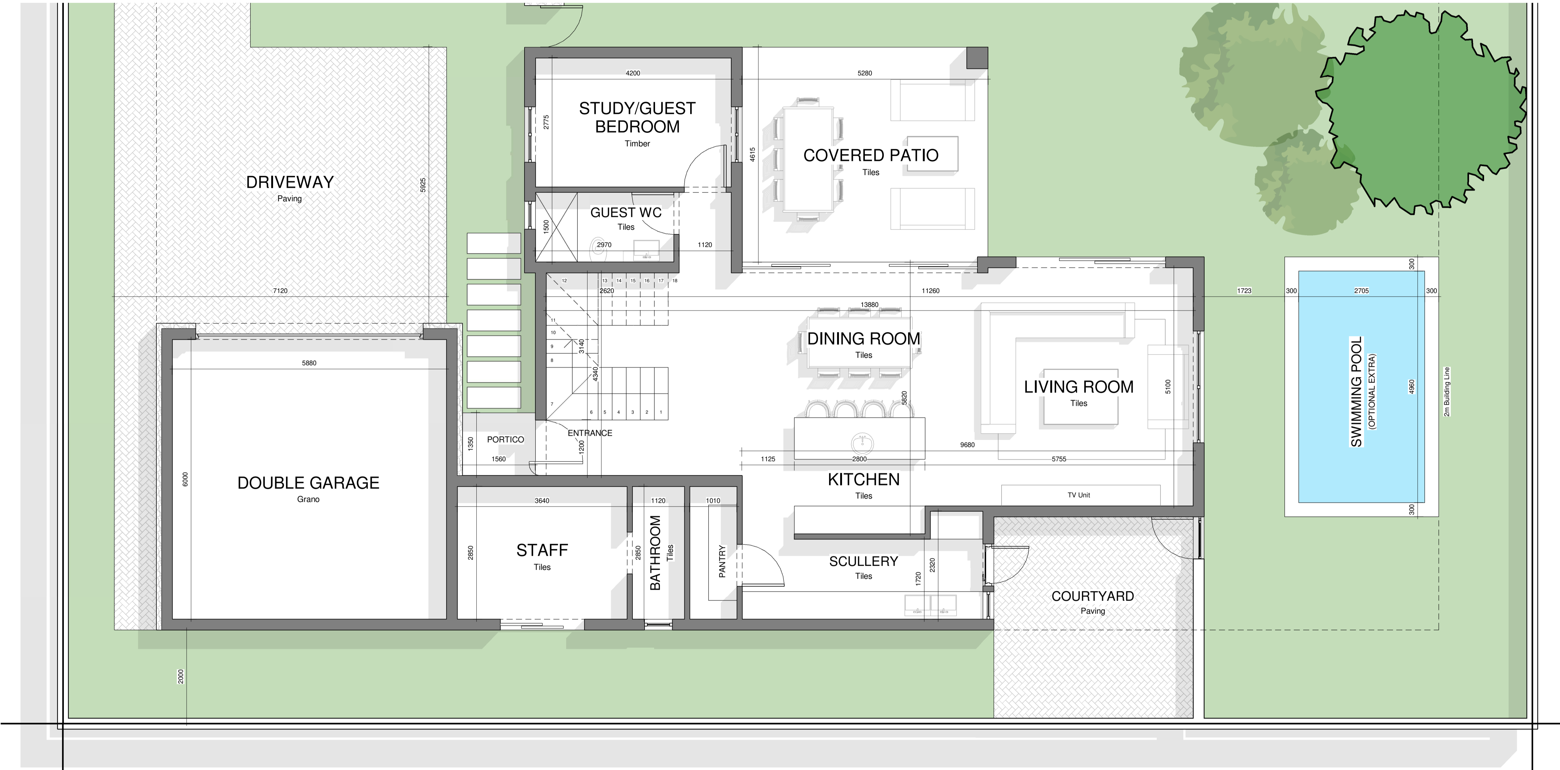
GROUND FLOOR_PTN 4 1 : 50
