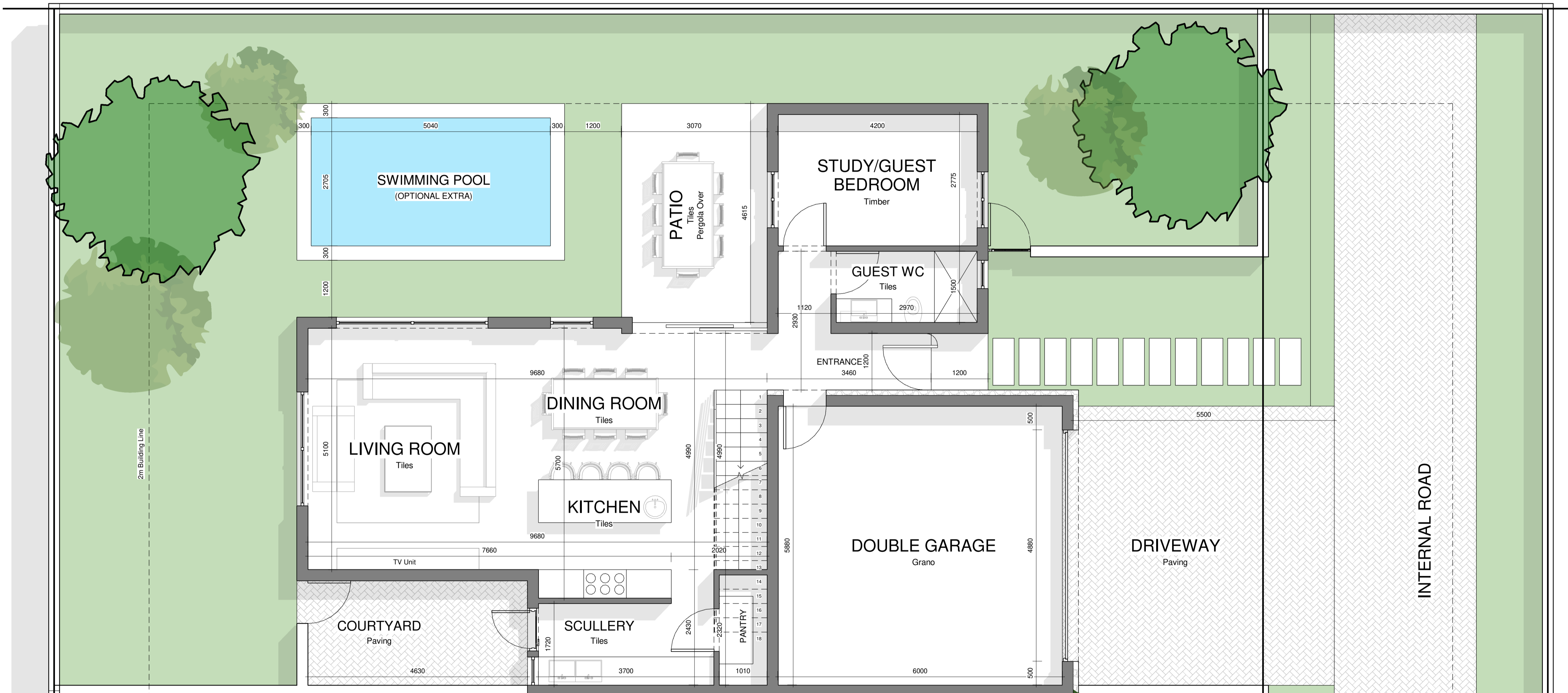
GROUND FLOOR - PTN 1 1 : 50
