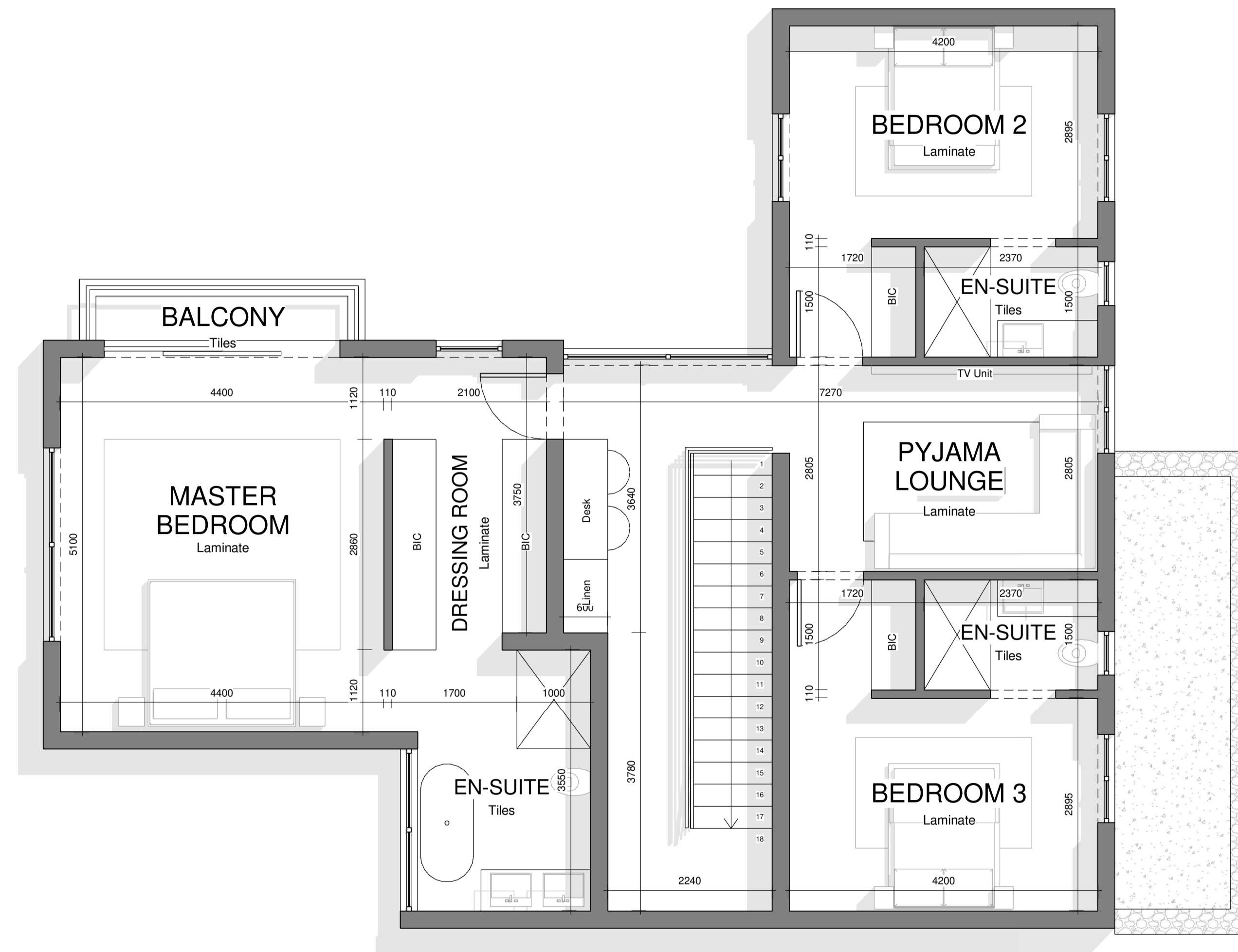
FIRST FLOOR - PTN 1 1 : 50
