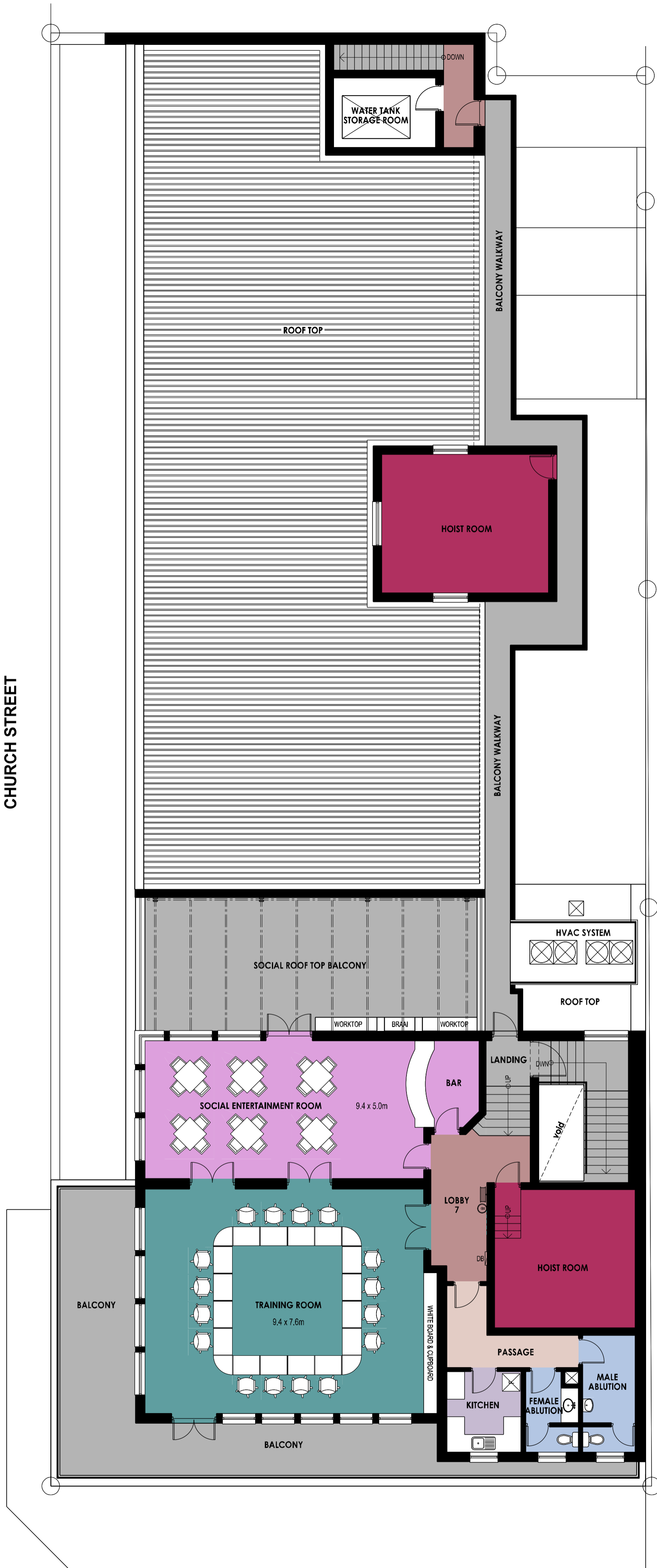
9 SEVENTH STOREY PLAN SCALE 1 : 100
